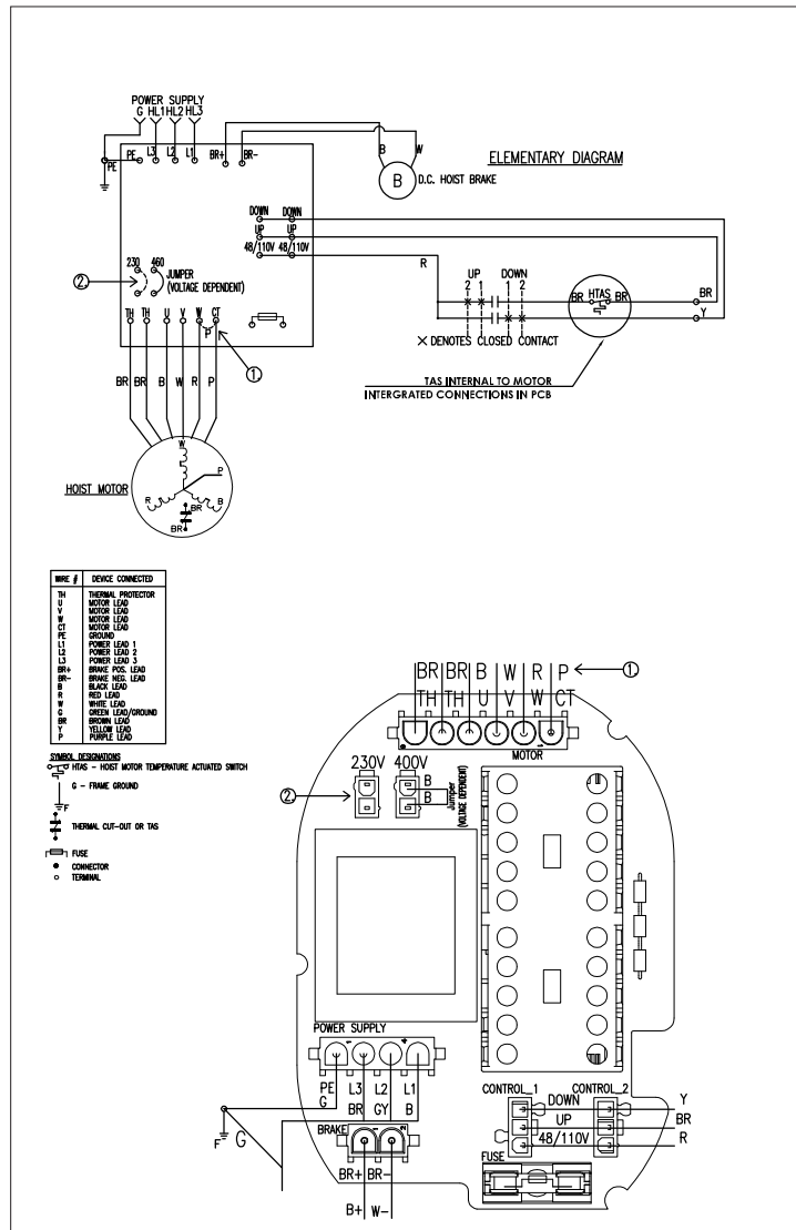
Figure 22 - 230-3-60, 400-3-50 PCB (Printed Circuit Board) Unit
