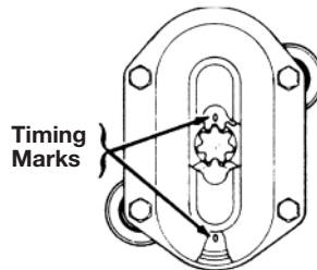
Figure 10 - Gear Timing
