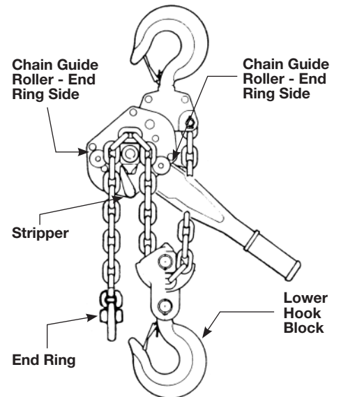
Figure 11 - Reeving - 6 Ton
