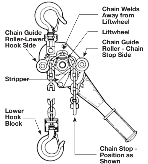
Chain Installation - 3/4, 1, 1 1/2, 2 and 3 Ton
