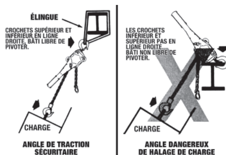
Figure 4 - Traction en angle
