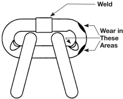
Figure 6 - Chain Inspection
