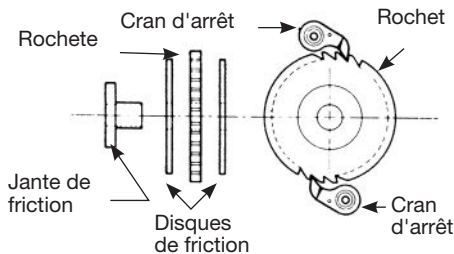
Figure 8 - Frein
