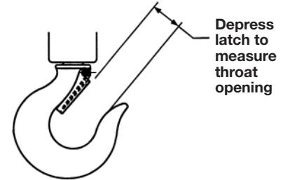
Figure 5 - Hook Inspection
