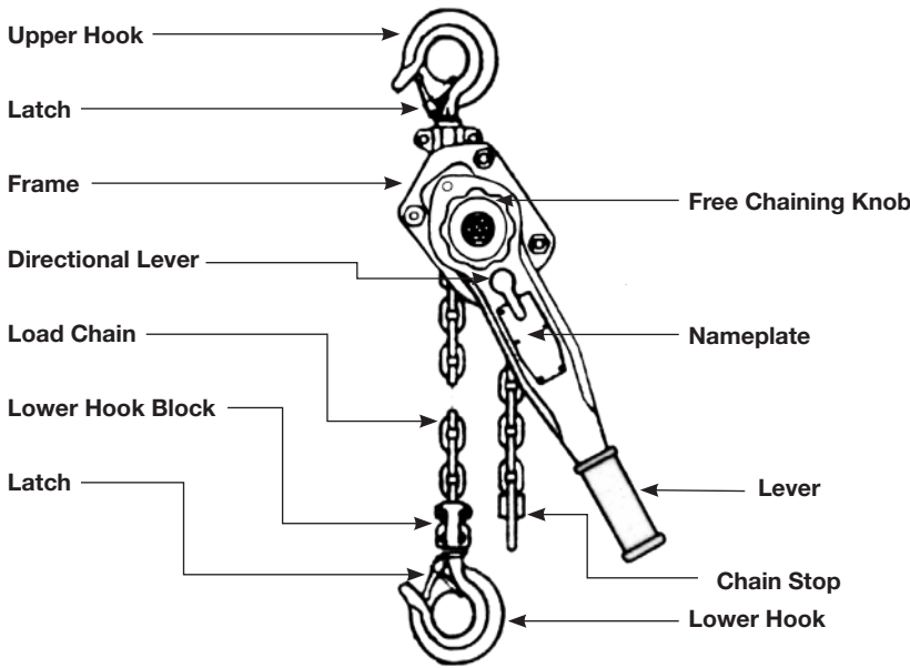
Figure 3 - Main Parts of Lever Hoist
