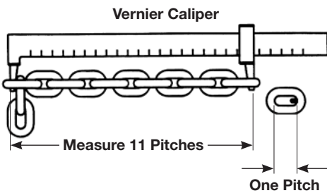
Figure 7 - Chain Inspection
