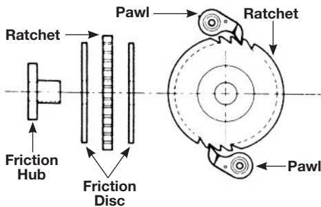
Figure 8 - Brake Assembly
