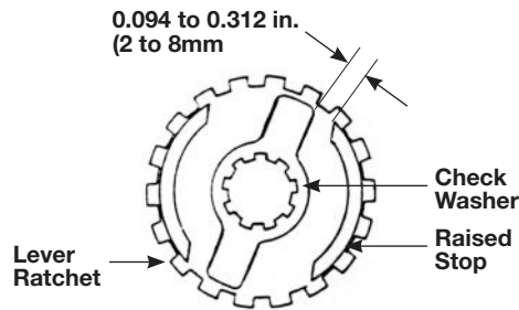
Figure 9 - Position of Check Washer
